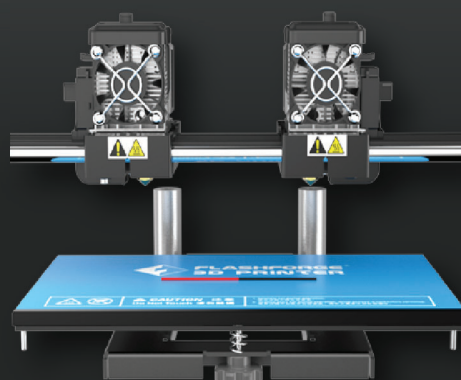
Y-Axis Calibration
